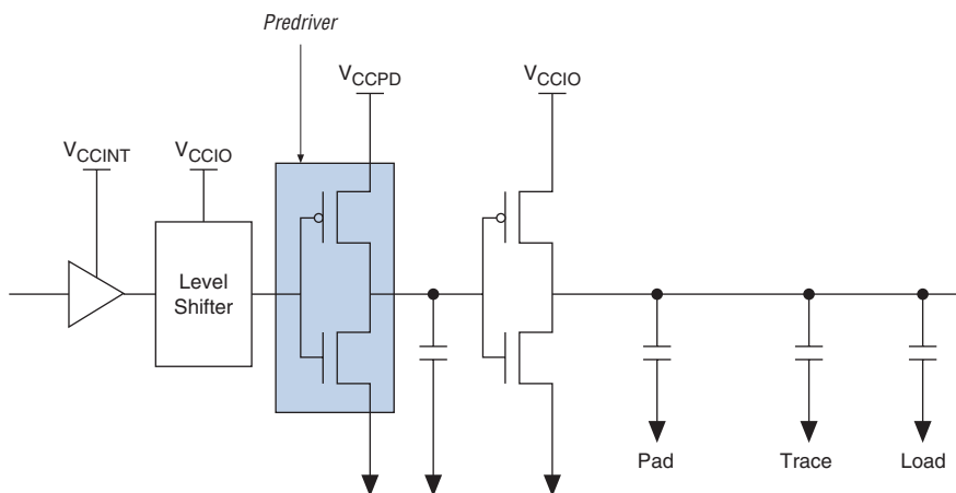
Figure 1. Stratix II I/O Buffer
